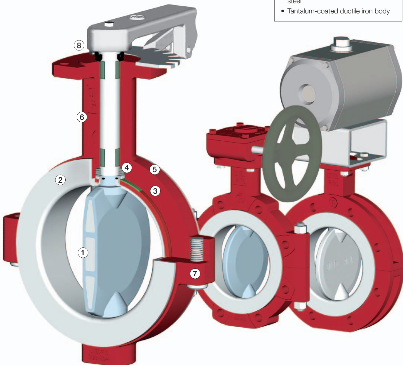
Wafer-style body NKS, NKS-C
